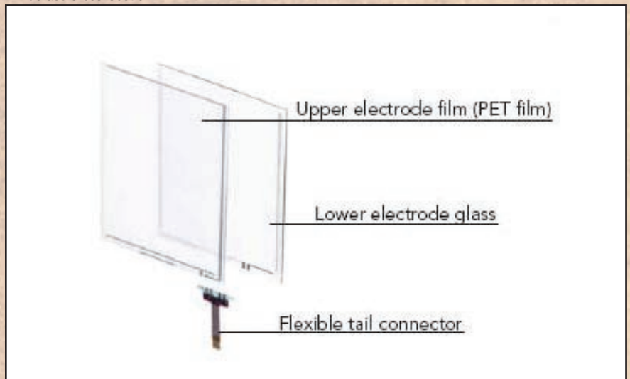
Film/Glass Cross-Section
