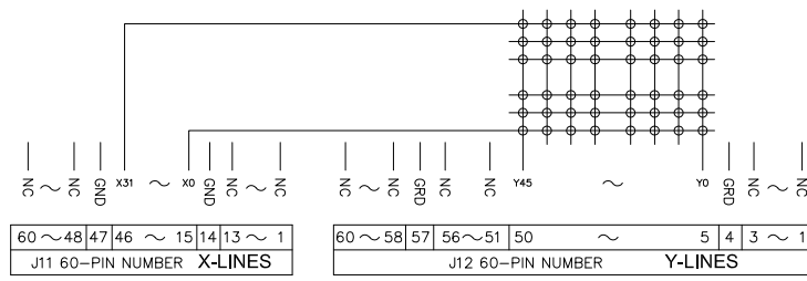
Key Matrix
